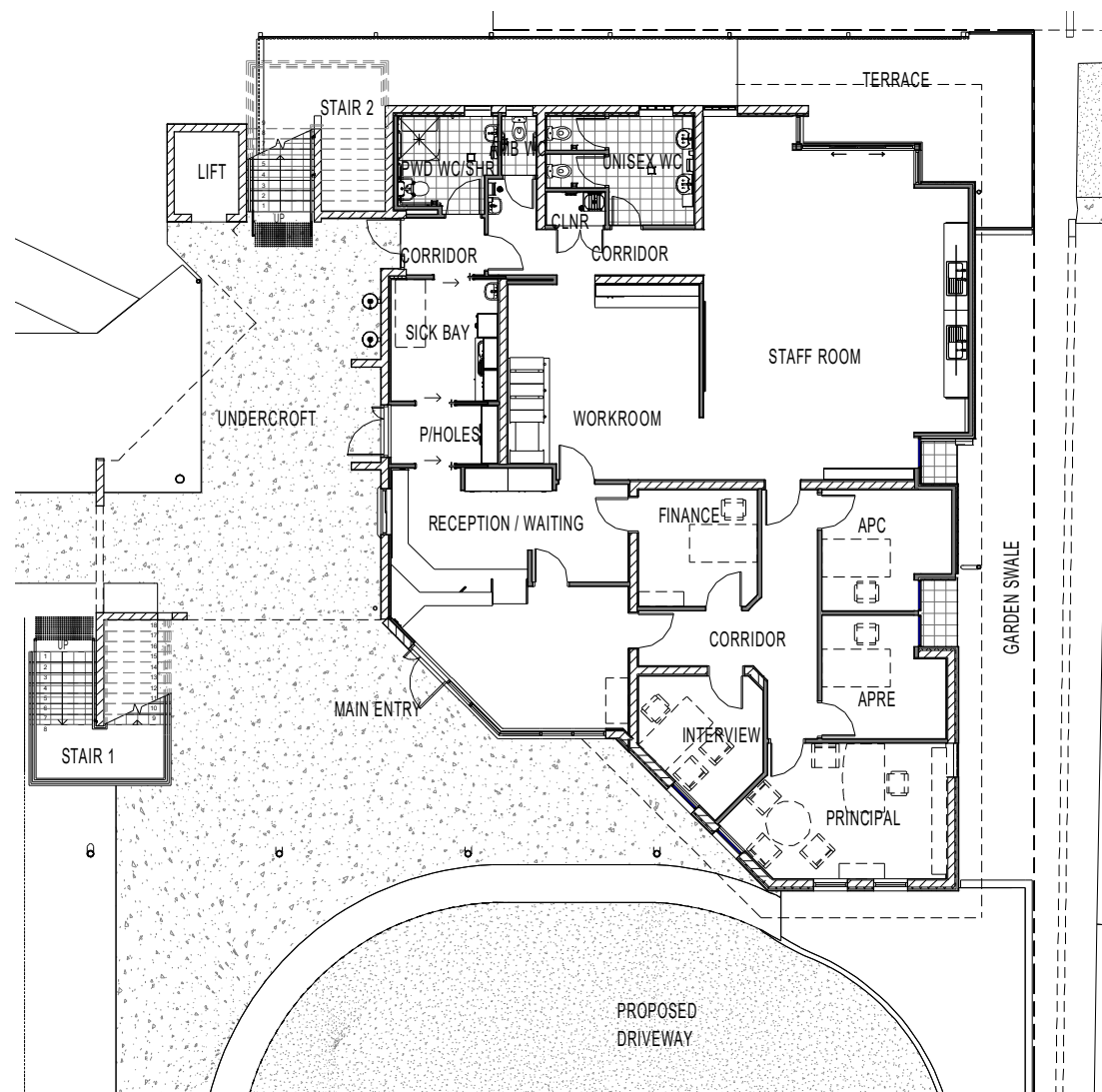
1 BLOCK F - GROUND FLOOR 1:100
